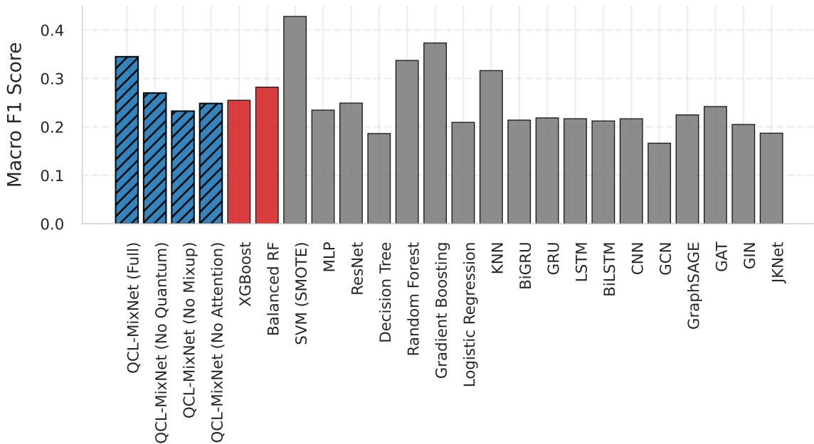
Performance on wine-quality-white
