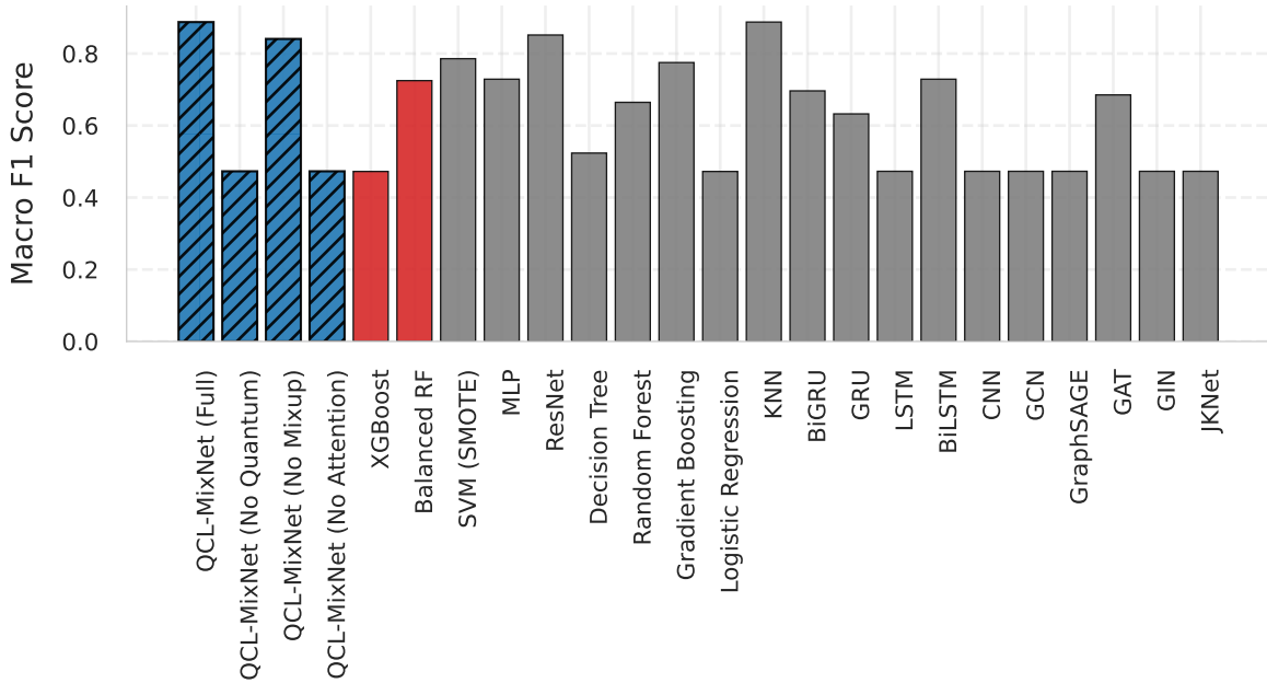
Performance on ecoli
