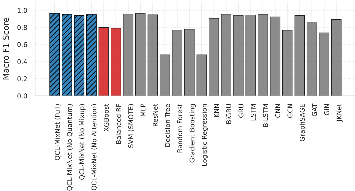
Performance on isolet
