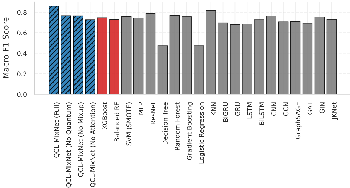
Performance on satimage
