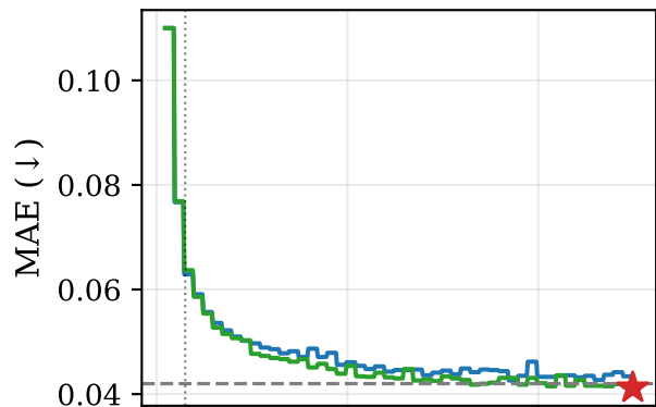
NL27K: MAE ( \downarrow )
