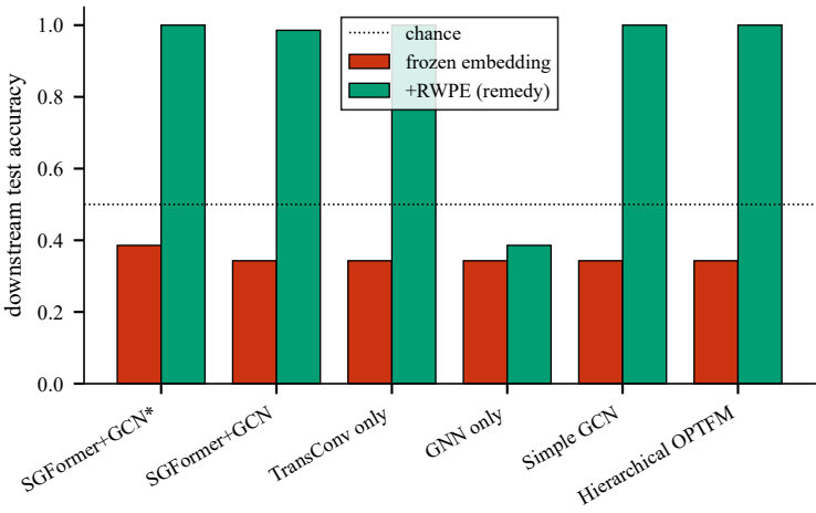
Connected-vs-disconnected: embedding ceiling and remedy
