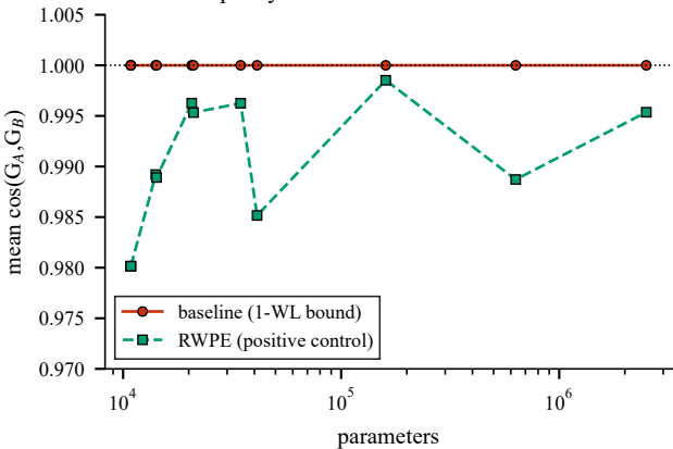
Capacity invariance of the 1-WL bound
