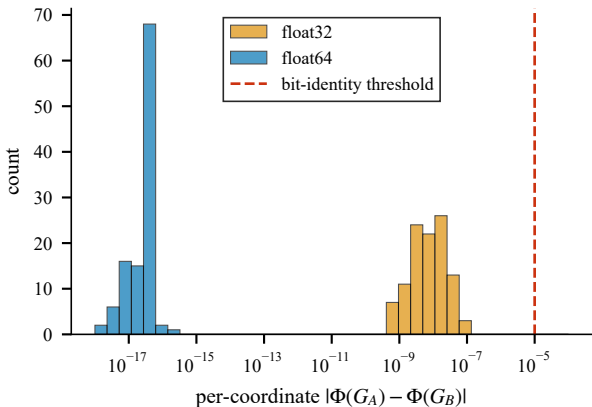
Embedding differences sit at machine epsilon
