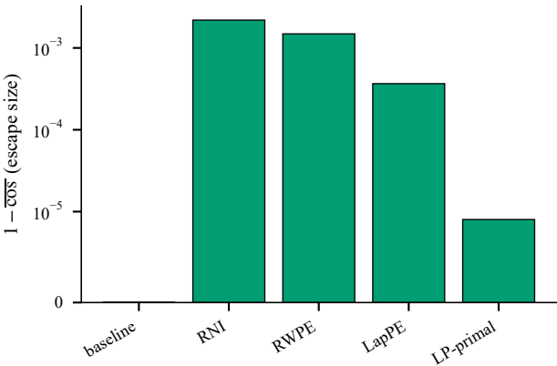
Which input encodings escape the bound
