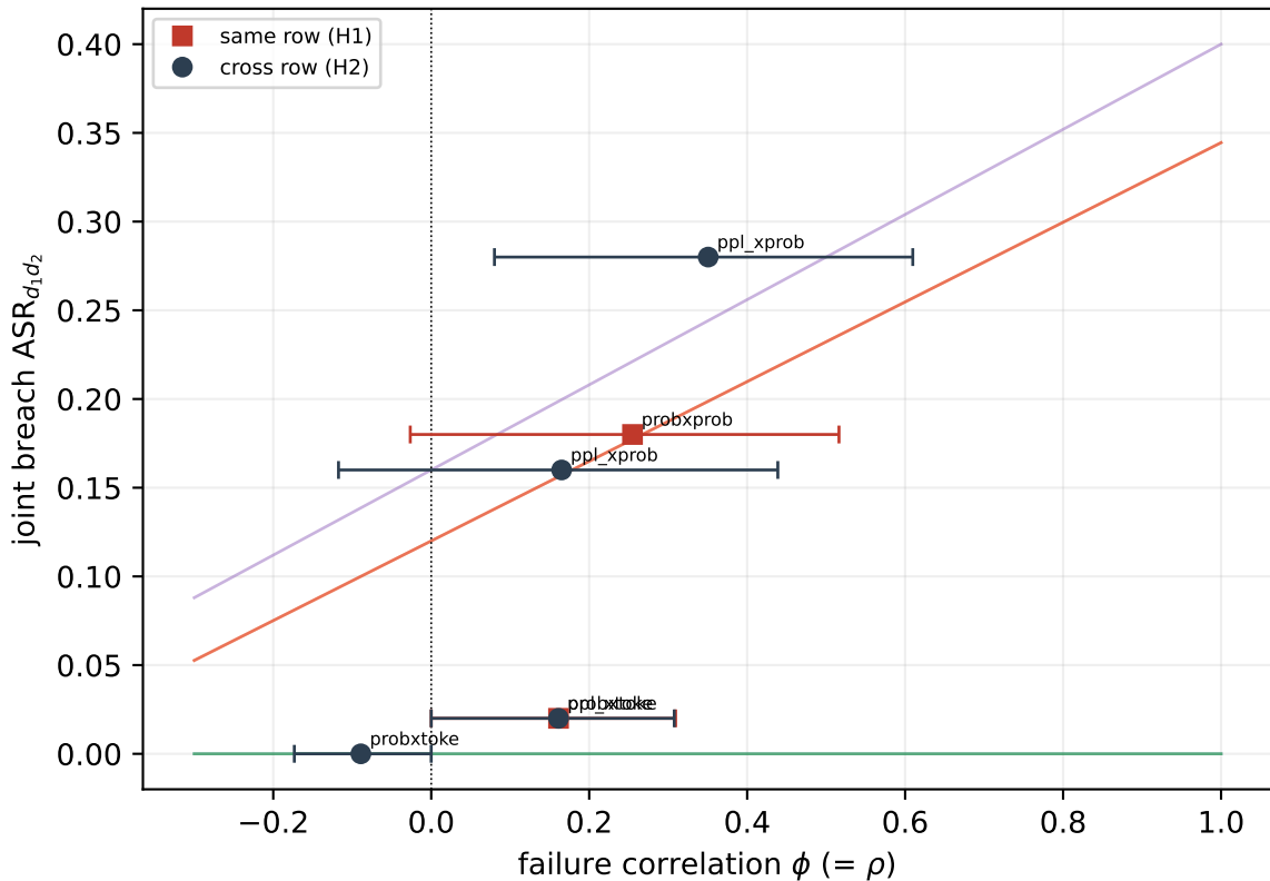
Figure 3(a): hpc_llama2_autodan
