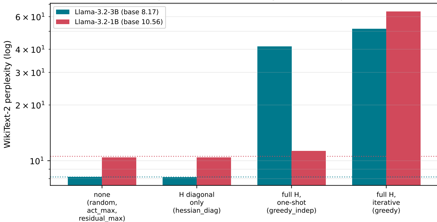
Damage requires the selector's off-diagonal Hessian coupling GPTQ-4 base, 2% protection, matched storage (dotted = unprotected base)
