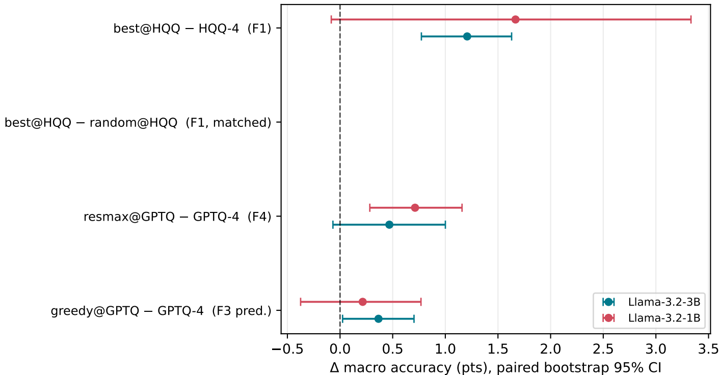
Downstream paired contrasts (F1 / F4 / F3)
