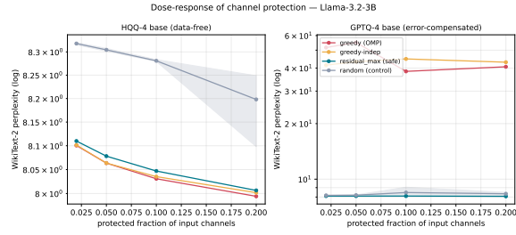
Figure 4: Perplexity against protection budget, Llama-3.2-3B, both bases.
