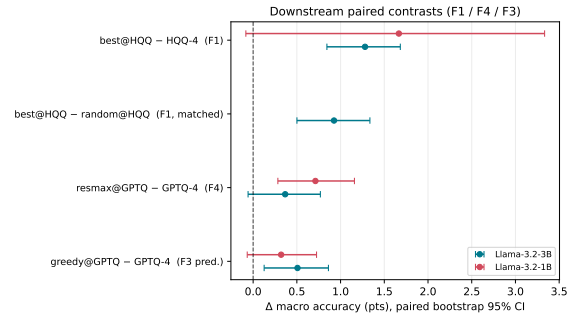
Figure 3: Downstream paired contrasts with 95% confidence intervals.
