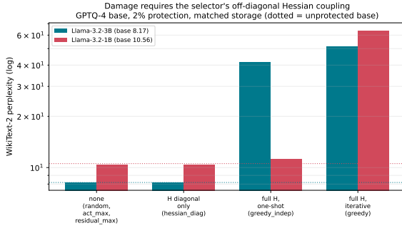
Figure 2: Perplexity by how much of the Hessian objective the selector uses. Dotted lines are the unprotected bases.
