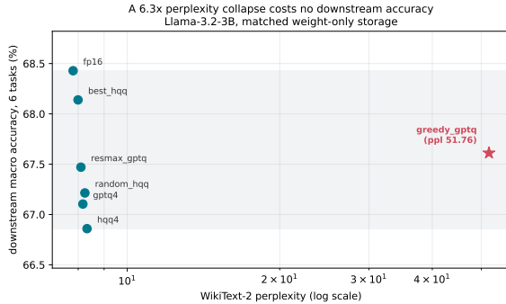
Figure 1: Every operating point of Llama-3.2-3B: WikiText-2 perplexity (log) against downstream macro accuracy. The catastrophic point sits 6.3 \times to the right yet at the same height, above both the GPTQ-4 and HQQ-4 bases.
