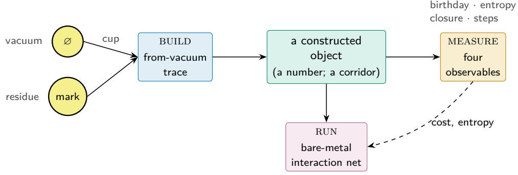
Figure 3: The engine in one line. Every object is built from the vacuum \emptyset and the mark it forces (the residue of the cup, \emptyset \rightarrow \tau \otimes \tau ), measured by four observables (one of them logical entropy), and lowered to (the engine runs) a bare-metal interaction net. This paper feeds one new object—the effective corridor—through the same stations, reaching the third as a lowering (Section 8).
