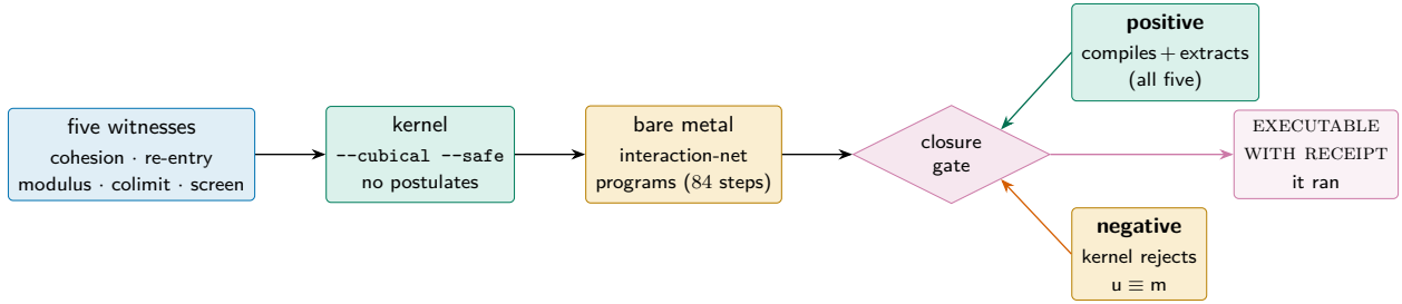
Figure 9: Closure as evidence of running, gated by a negative control. The five witnesses pass the kernel, lower to bare-metal interaction-net programs, and are admitted as executable closure only by a gate carrying both a positive control (genuine compilation and extraction) and a negative control (the kernel provably rejects the degenerate collapse u \equiv m ). A degenerate witness cannot pass the gate that admits the genuine one (Theorem 8.1).
