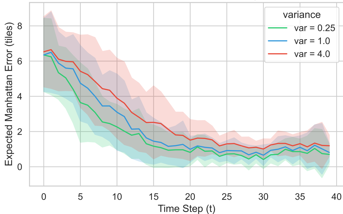
Effect of Sensor Variance on Quality Error
