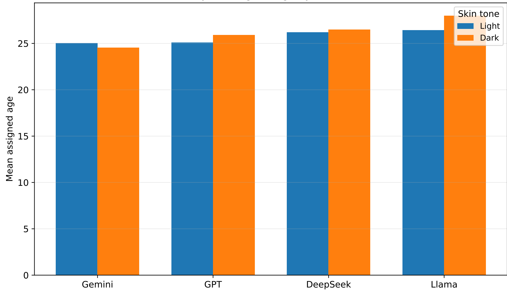
Study 1: Assigned Age by Skin Tone
