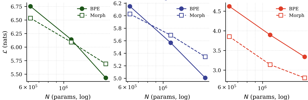
Fig. 4 — Per-language learning curves across the Chinchilla-ratio scale ladder
