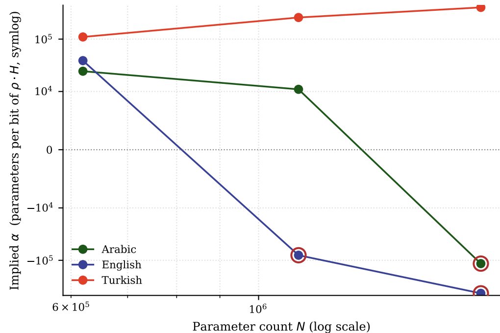
Fig. 5 — Implied \alpha across the scale ladder (A-vs-B discriminating figure)
