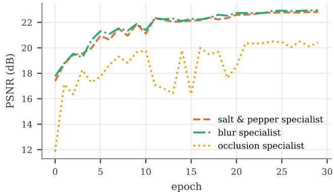
(b) T2 specialists, validation PSNR on own corruption
