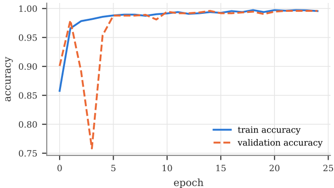
(a) T2 corruption classifier
