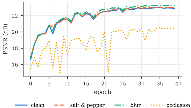
(b) T1 validation PSNR by input condition
