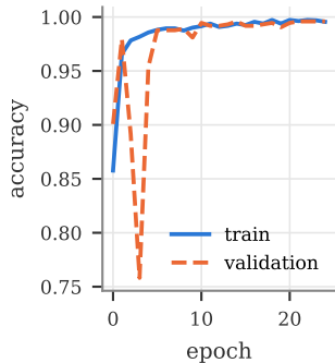
(a) T2 classifier accuracy
