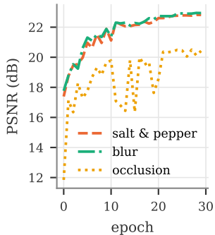
(b) T2 specialists, val. PSNR
