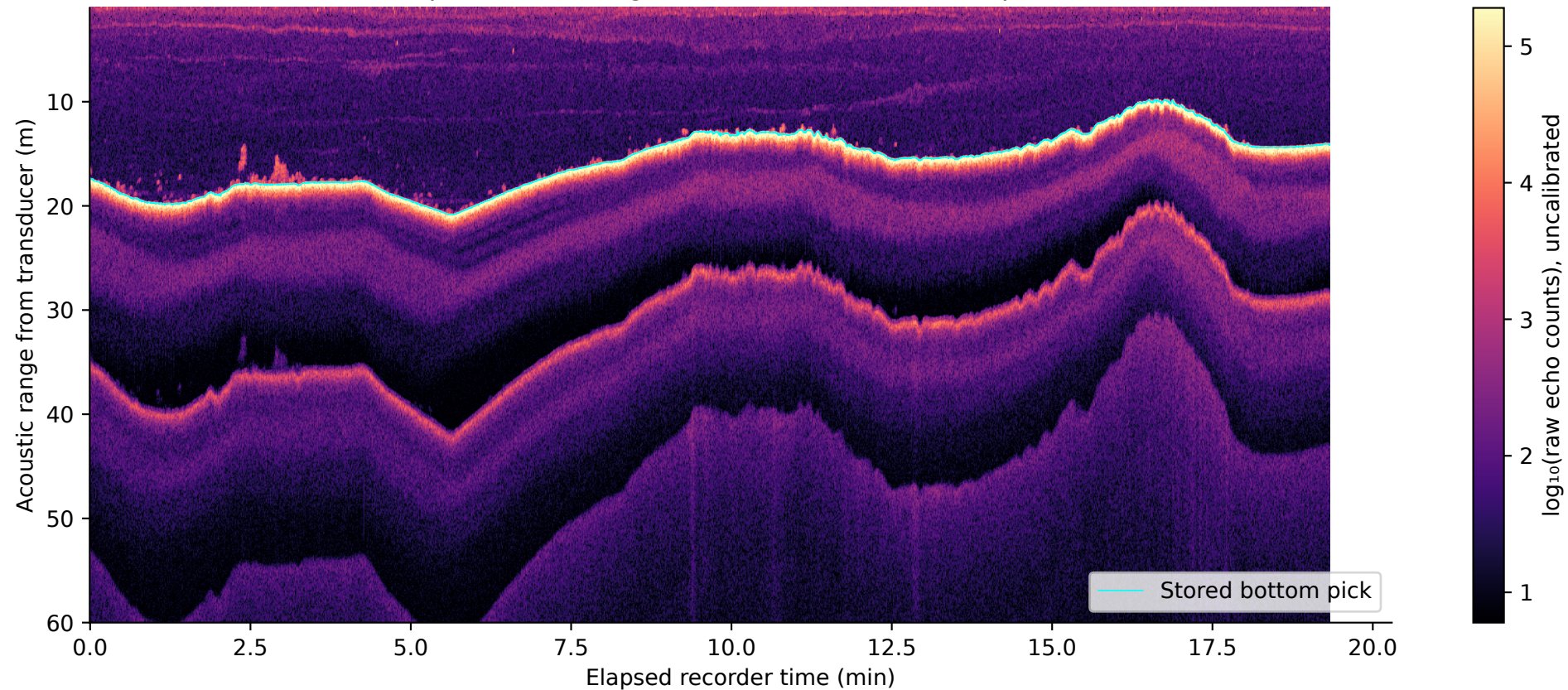
Split-beam echogram with recorded bottom picks
