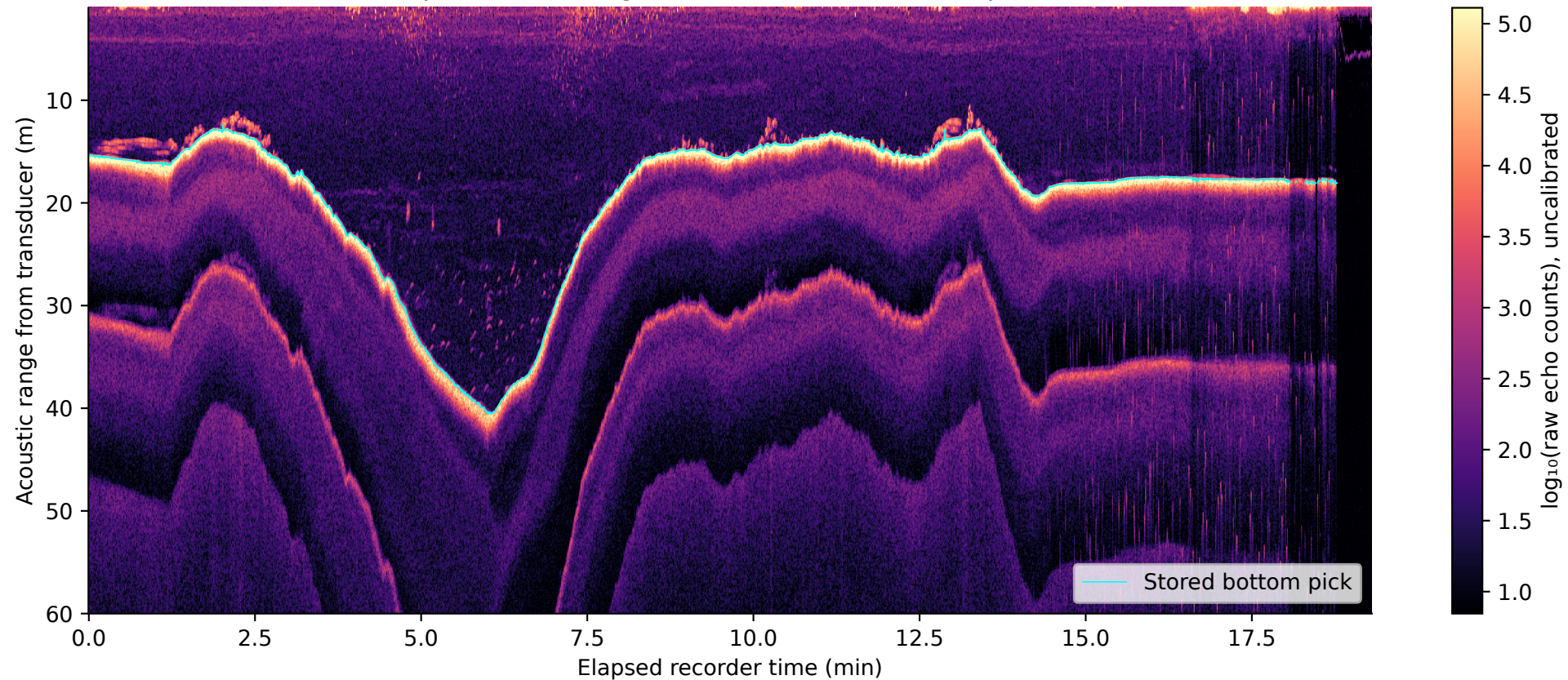
Split-beam echogram with recorded bottom picks
