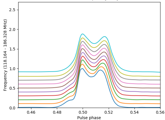
Profile evolution with frequency for J0700+6418
