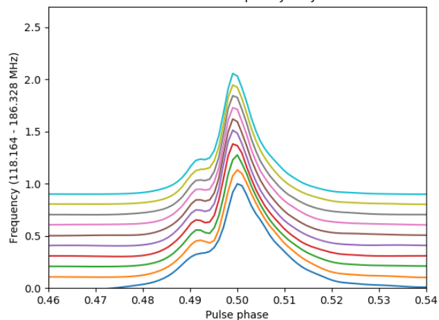
Profile evolution with frequency for J1955+5059
