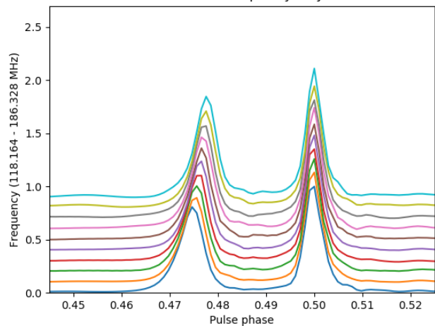
Profile evolution with frequency for J0921+6254
