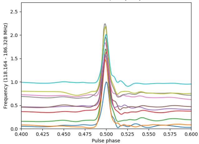
Profile evolution with frequency for J0546+2441
