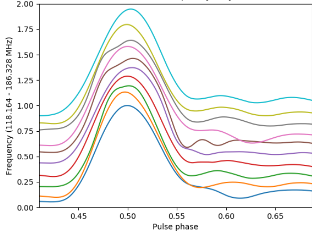
Profile evolution with frequency for J0700+6418
