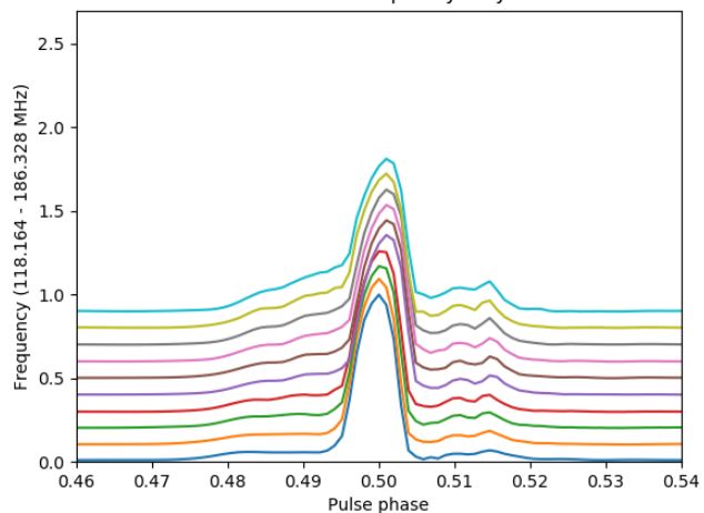
Profile evolution with frequency for J1840+5640
