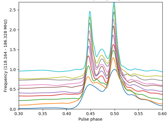
Profile evolution with frequency for J0102+6537
