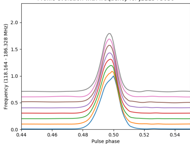
Profile evolution with frequency for J1115+5030
