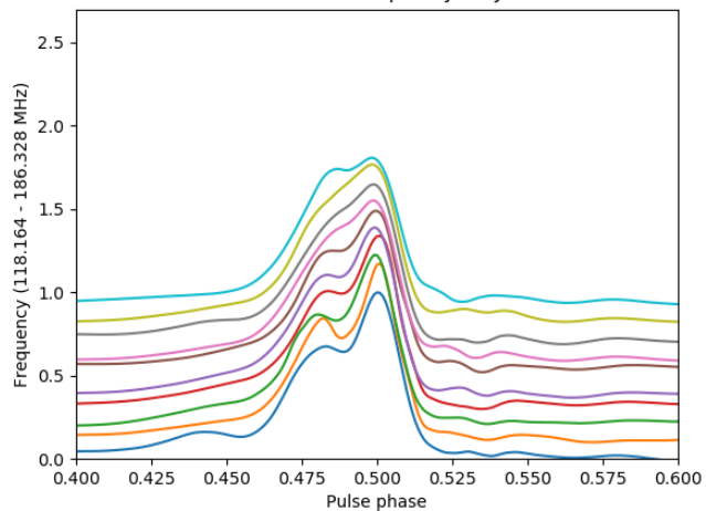
Profile evolution with frequency for J0815+4611
