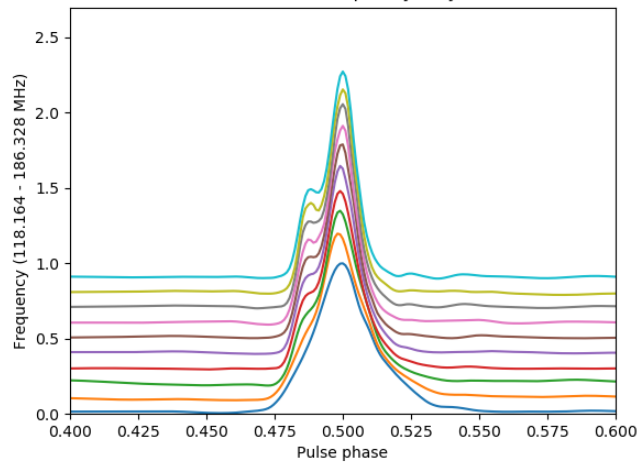
Profile evolution with frequency for J0540+3207
