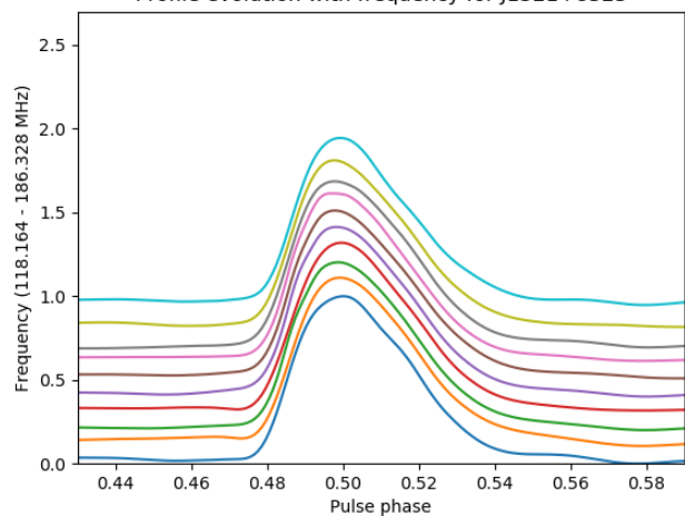
Profile evolution with frequency for J1321+8323
