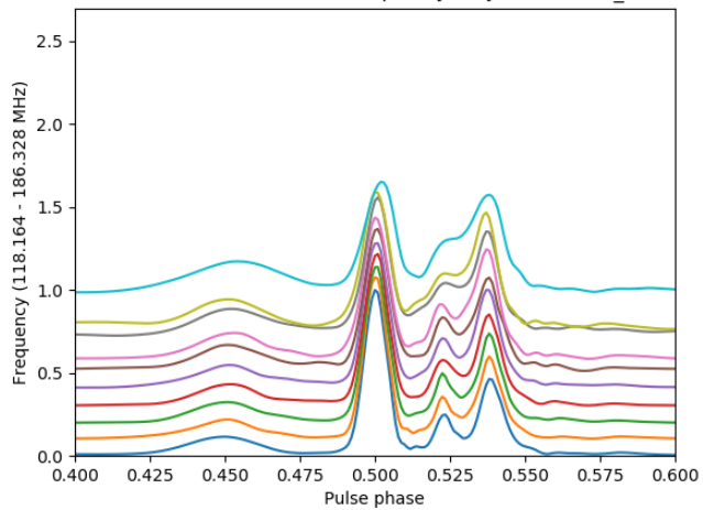
Profile evolution with frequency for J0051+0423_
