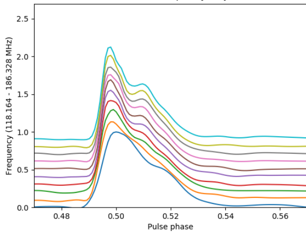
Profile evolution with frequency for J0335+4555
