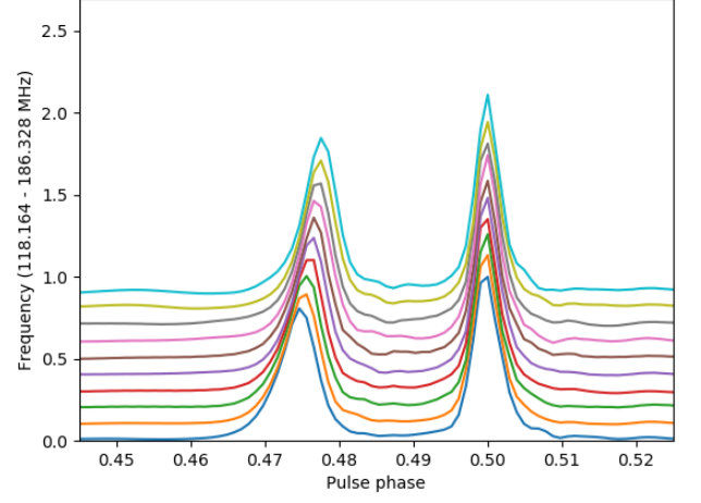
Profile evolution with frequency for J0921+6254
