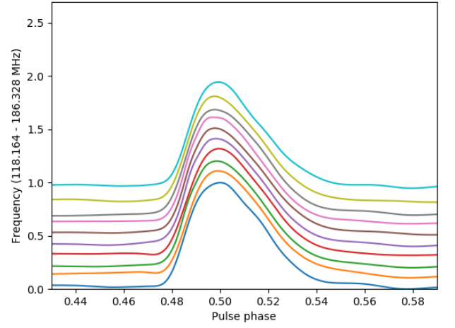
Profile evolution with frequency for J1321+8323
