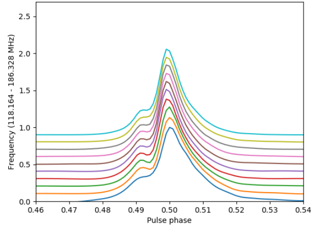
Profile evolution with frequency for J1955+5059
