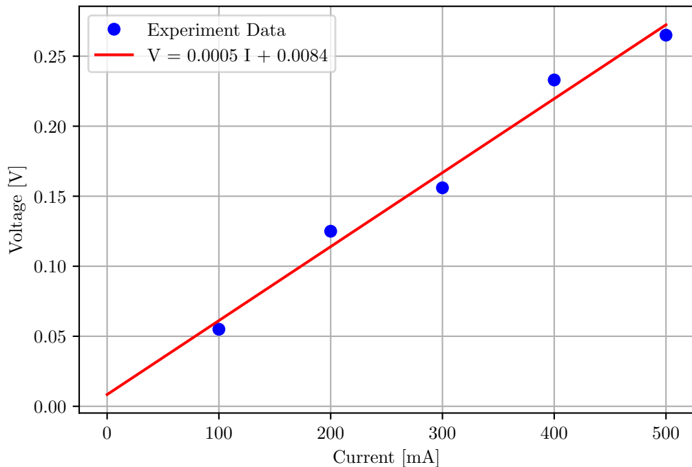
Graph of Voltage as a Functions of Current
