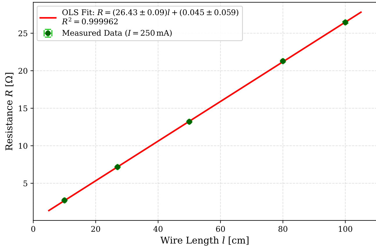
Resistance vs. Wire Length ( R - l )
