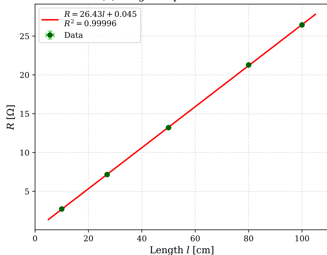
(b) Length Dependence: R vs. l
