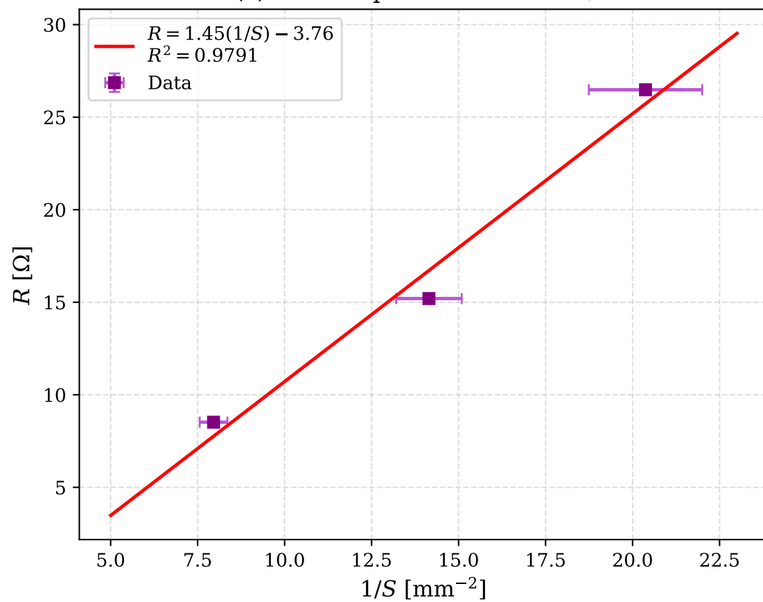
(c) Area Dependence: R vs. 1/S
