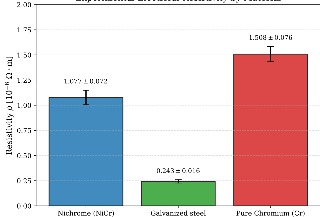
Experimental Electrical Resistivity by Material
