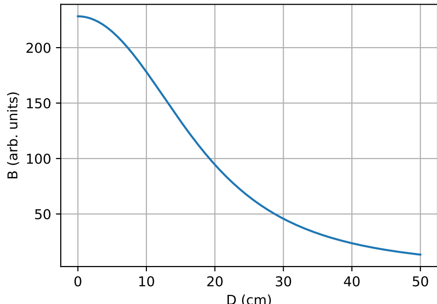
Theoretical B(D) for a = R/2
