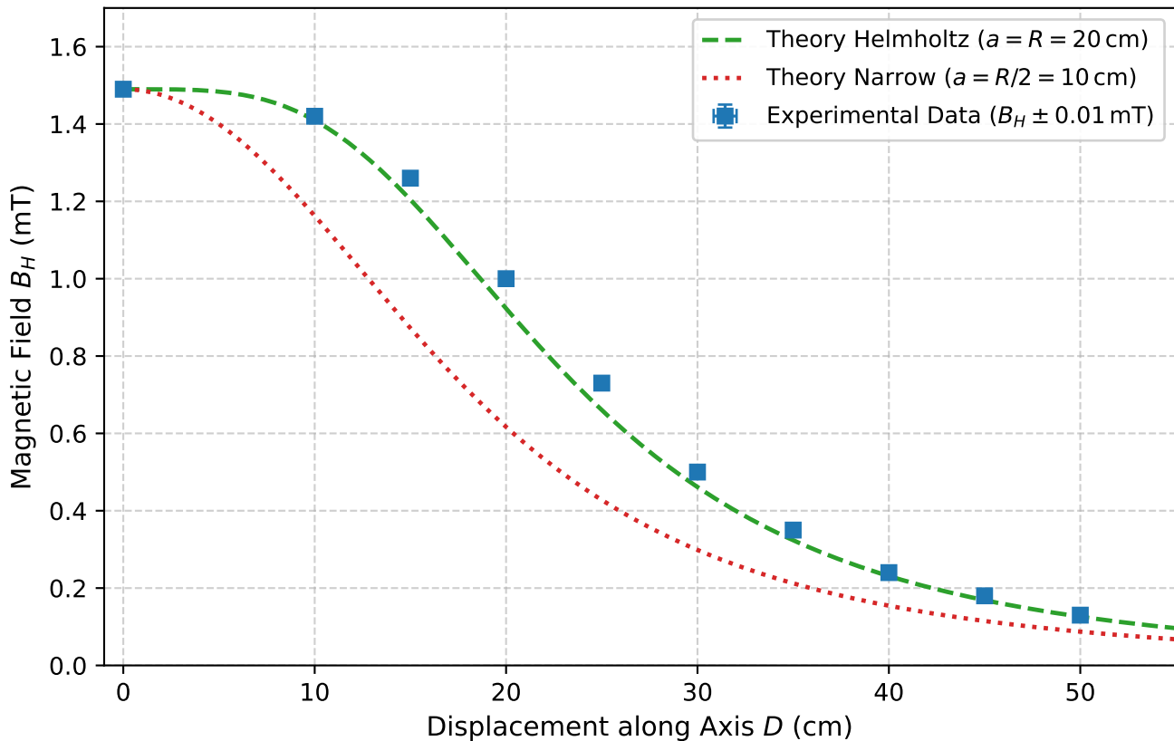
Axial Magnetic Field Distribution of Helmholtz Coils
