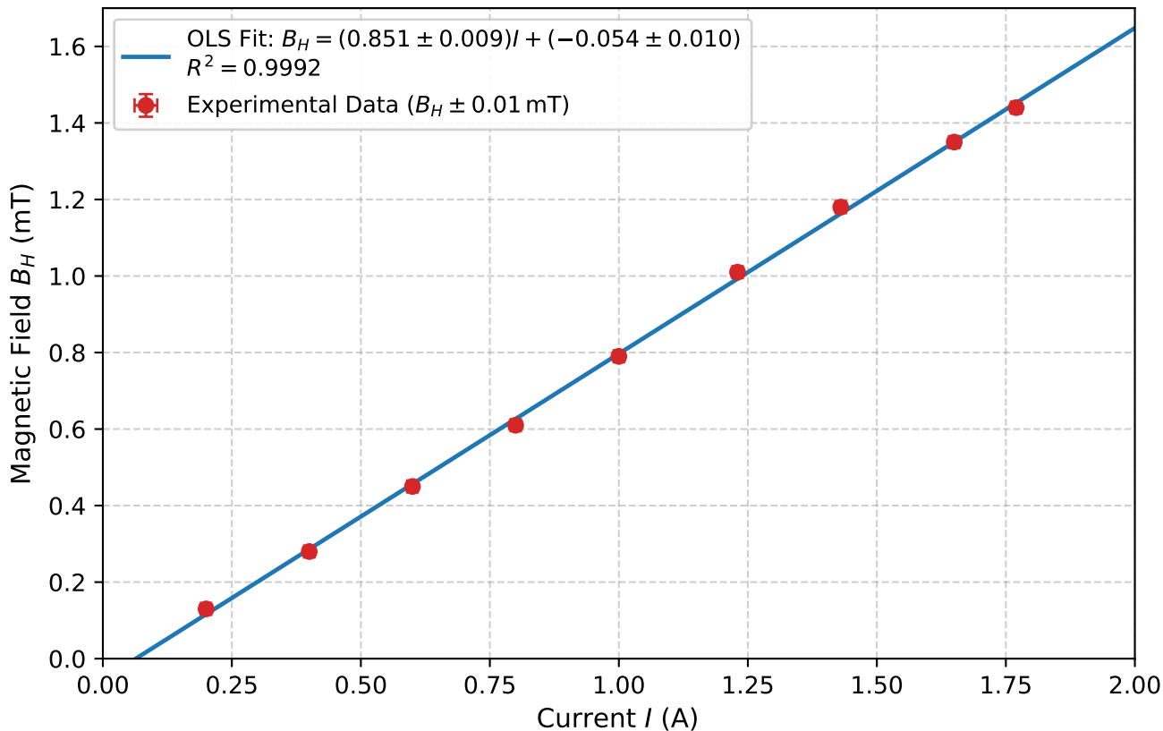
Magnetic Field vs Coil Current ( B_H vs I )
