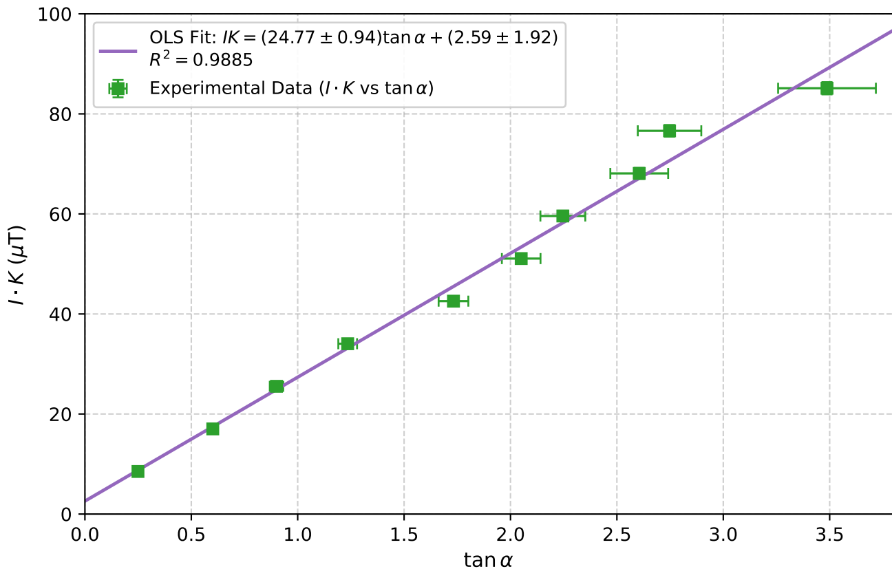
Tangent Galvanometer: I \cdot K vs \tan \alpha
