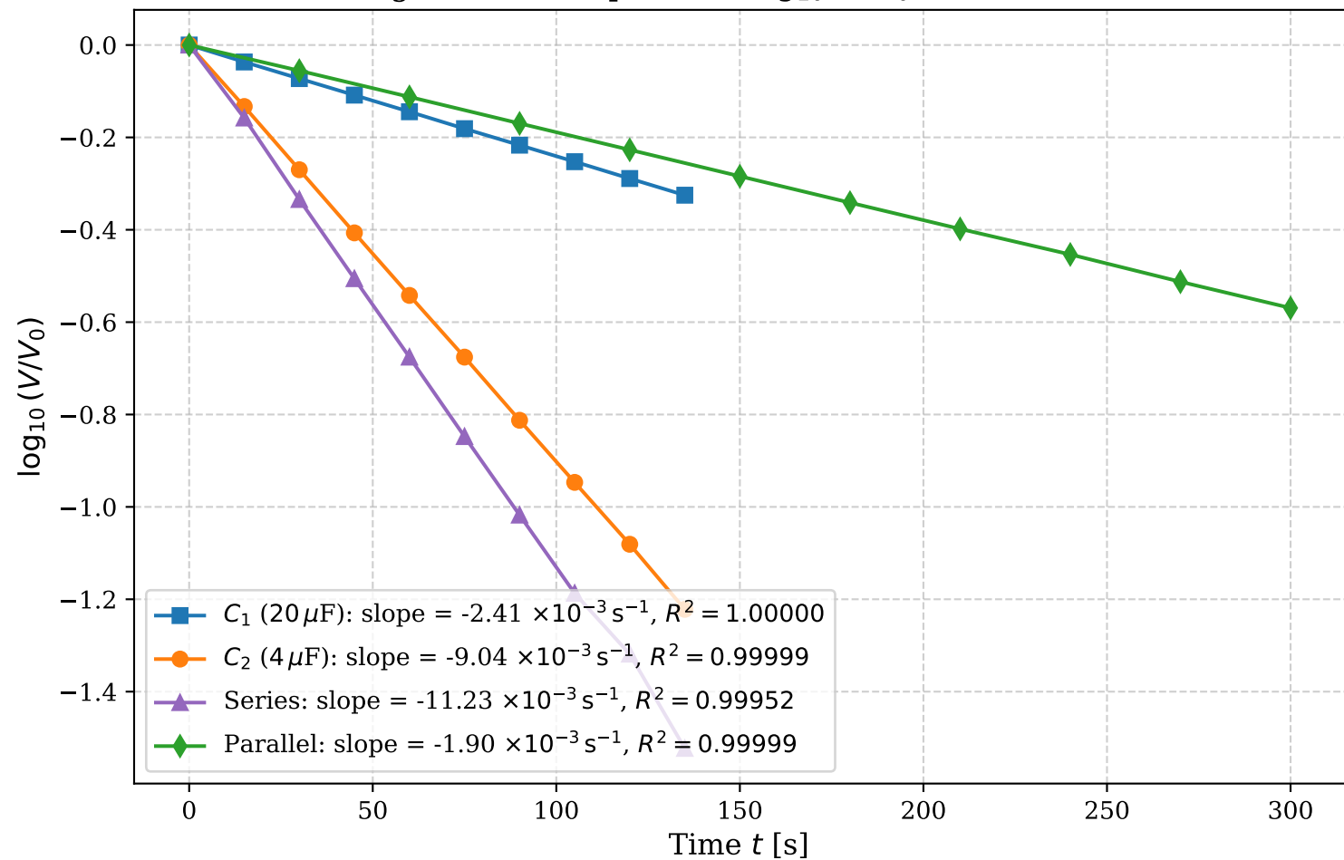
Linear Regression Comparison: \log_{10}(V/V_0) vs. t for All Circuits
