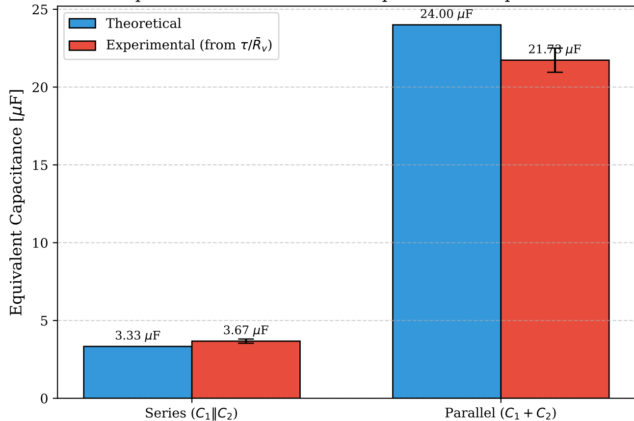
Comparison of Theoretical vs. Experimental Capacitances
