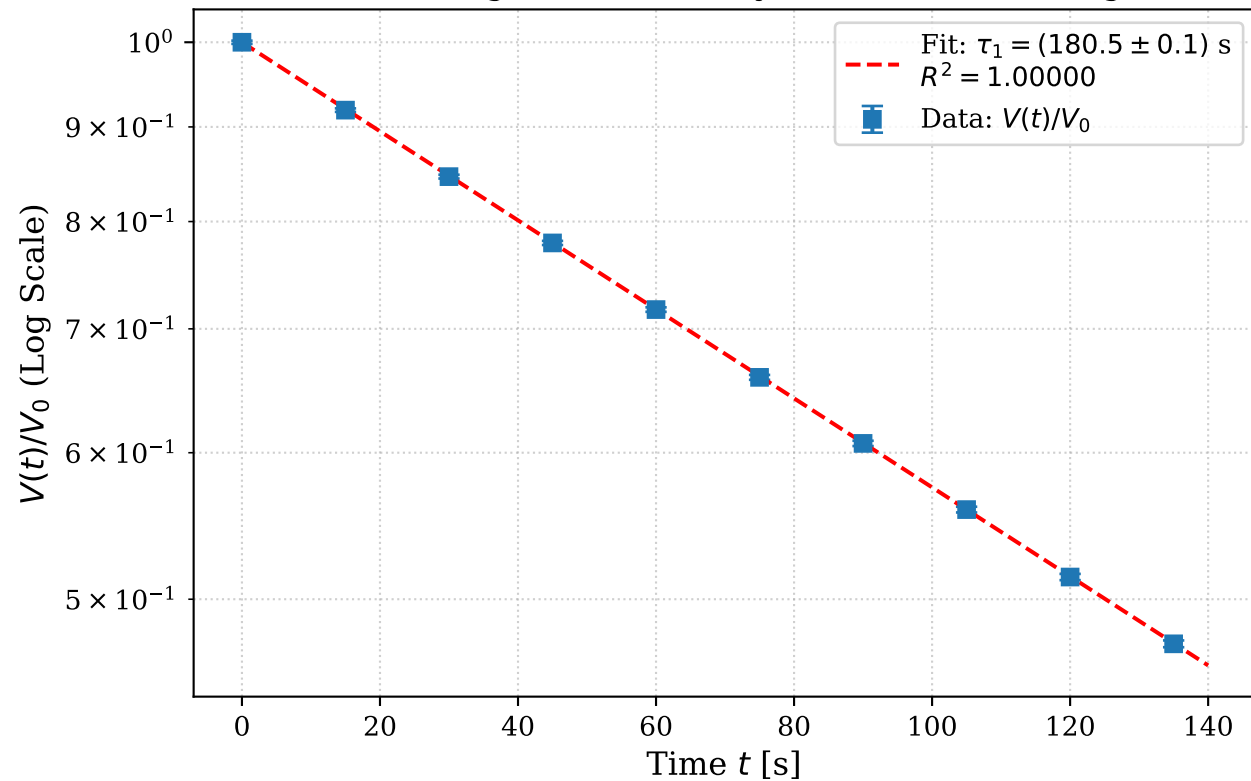
(a) Semilogarithmic Decay of Voltmeter Voltage
