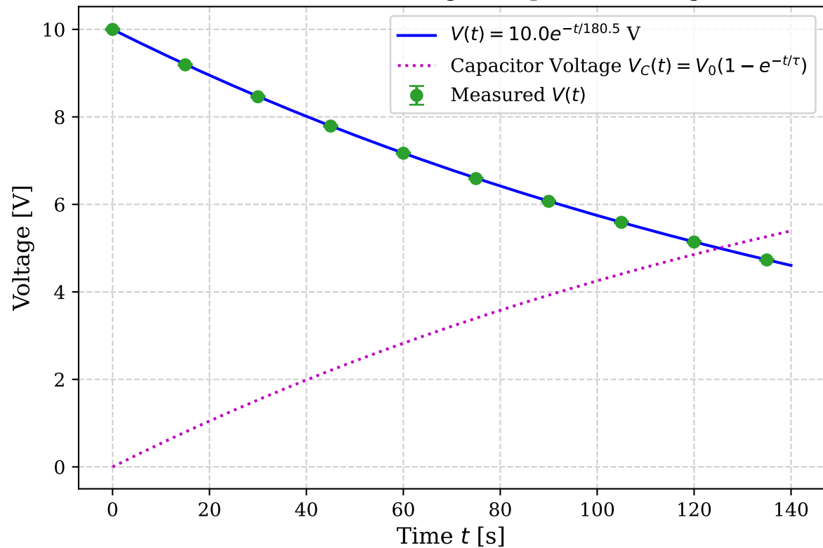
(b) Voltmeter Reading & Capacitor Voltage
