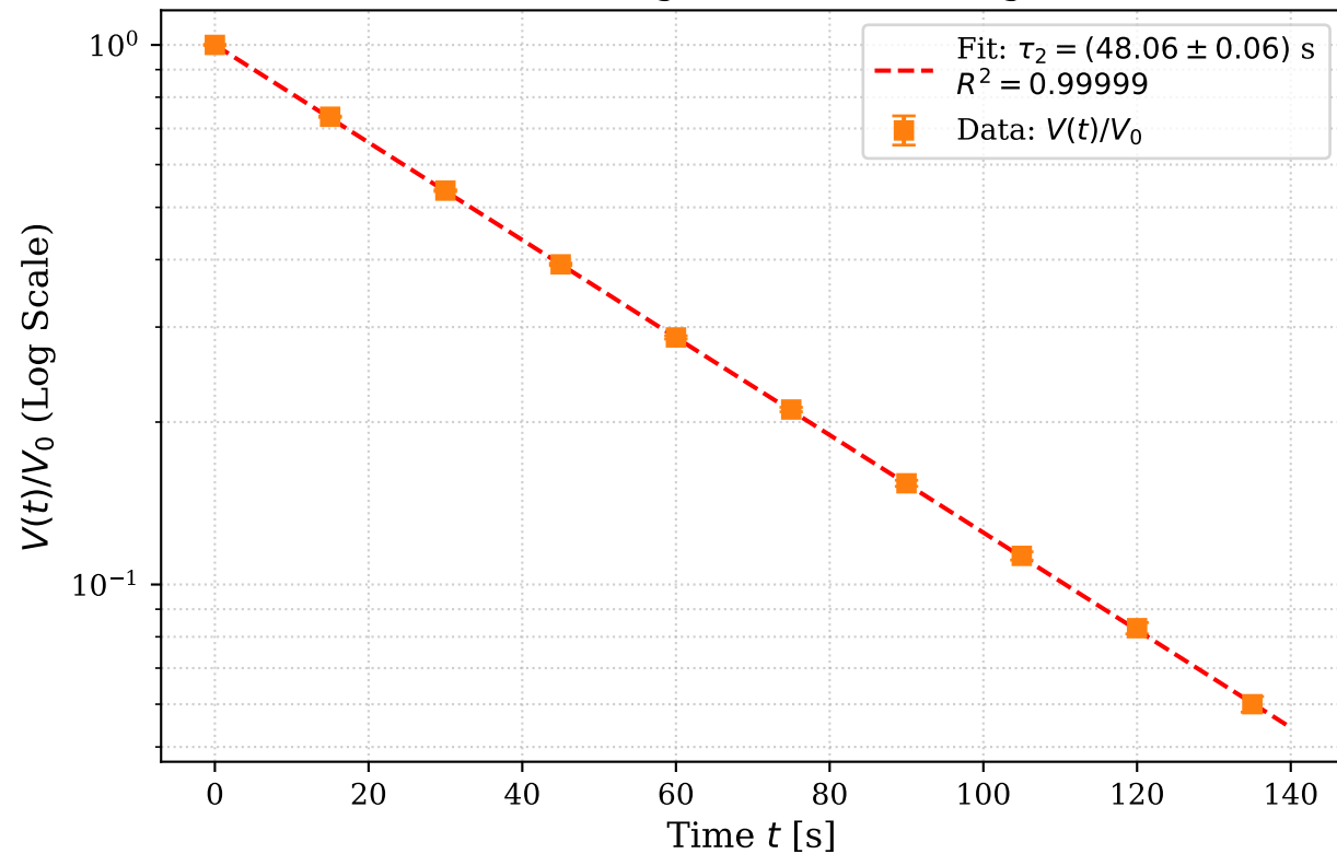
(a) Semilogarithmic Discharge
