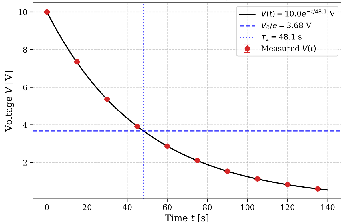
(b) Exponential Discharge Curve
