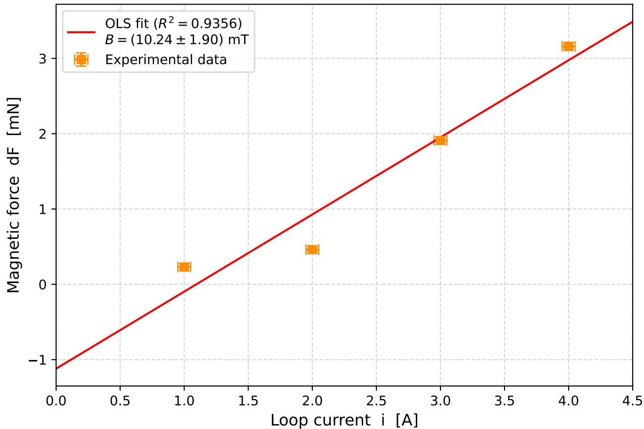
DeltaF vs i (L=10cm, I m =2A)
