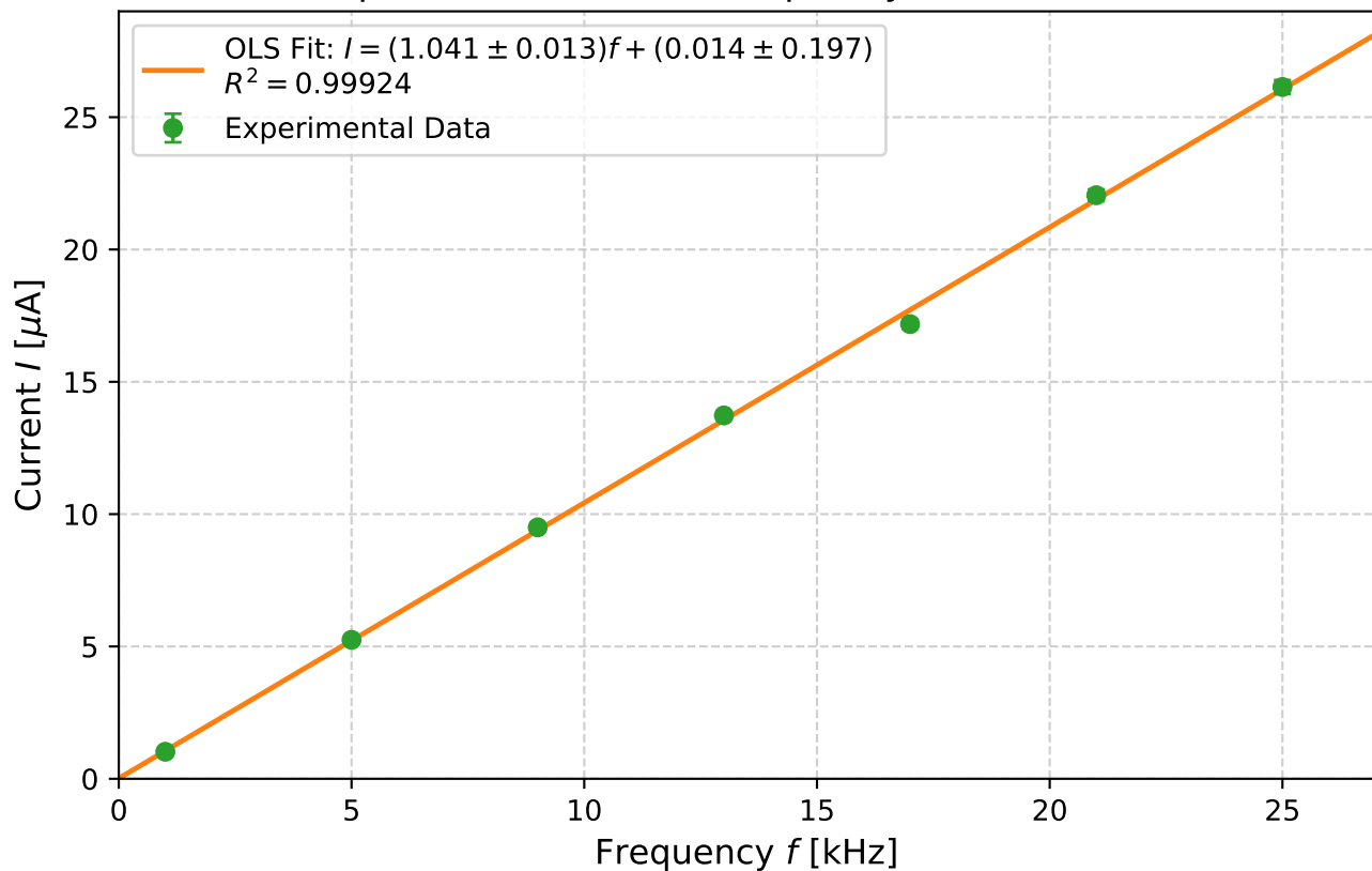
Capacitor Current vs. Frequency (Air Dielectric)
