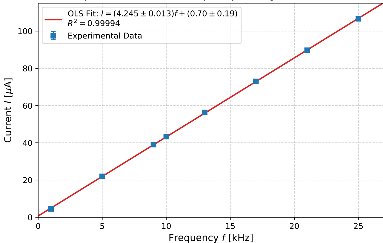
Capacitor Current vs. Frequency (Plexiglass Dielectric)
