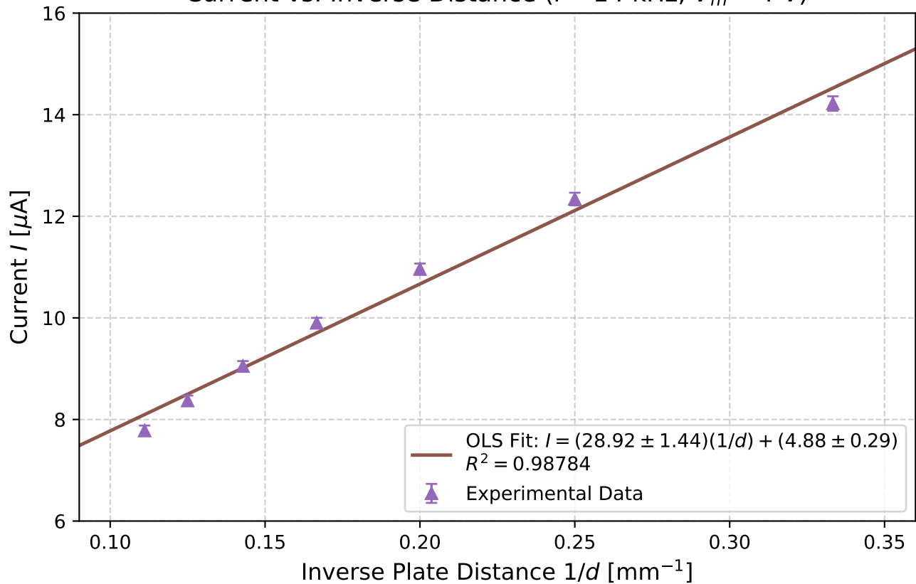
Current vs. Inverse Distance ( f = 14 kHz, V_m = 4 V)
