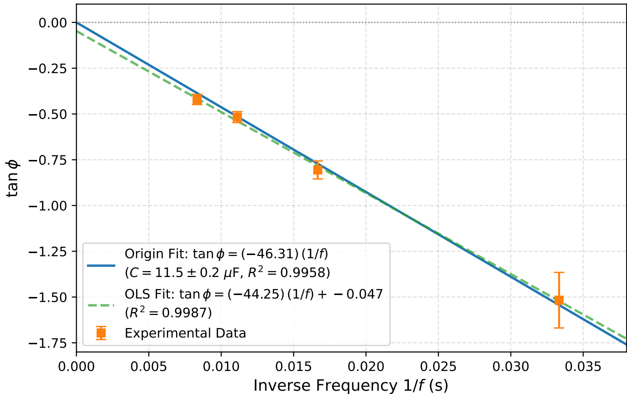
RC Series Circuit: \tan \phi vs. 1/f ( R = 300 \, \Omega )
