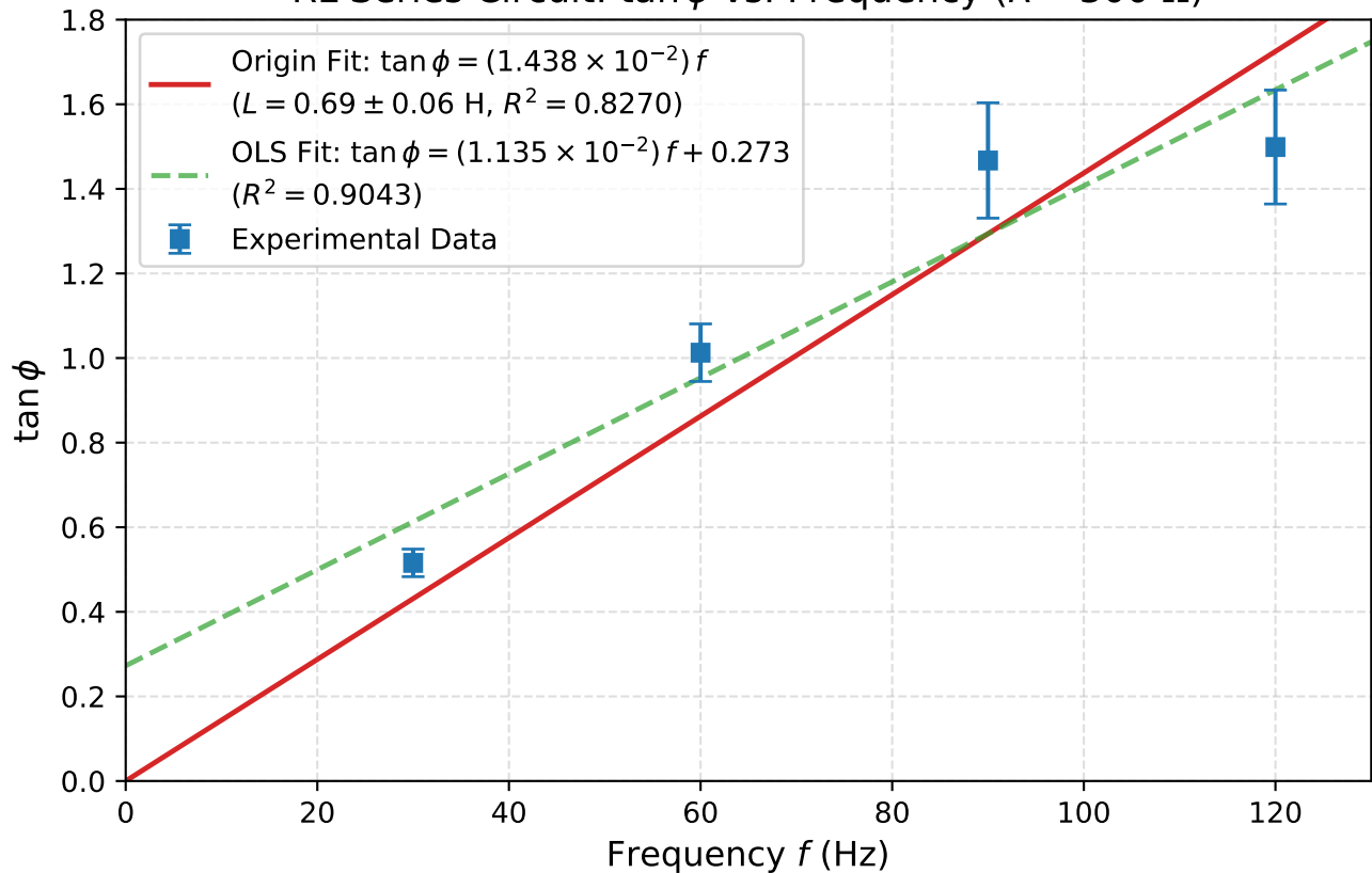
RL Series Circuit: \tan \phi vs. Frequency ( R = 300\ \Omega )
