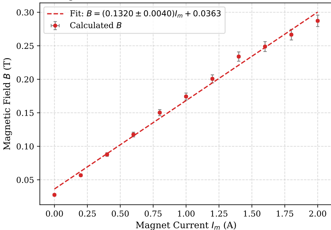
Magnetic Field Calibration Curve with Error Bars
