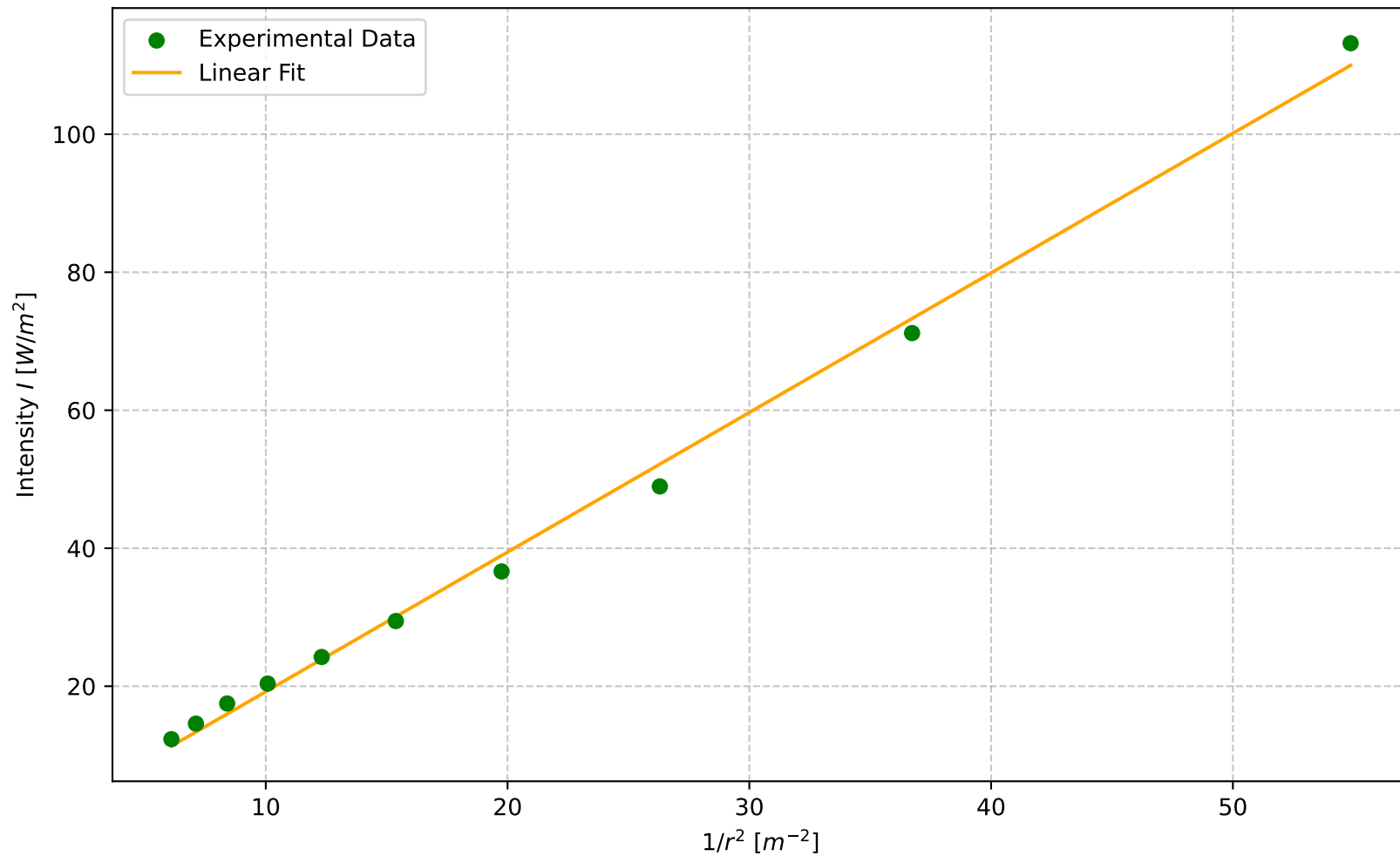
Inverse Square Law: Intensity vs. 1/r^2
