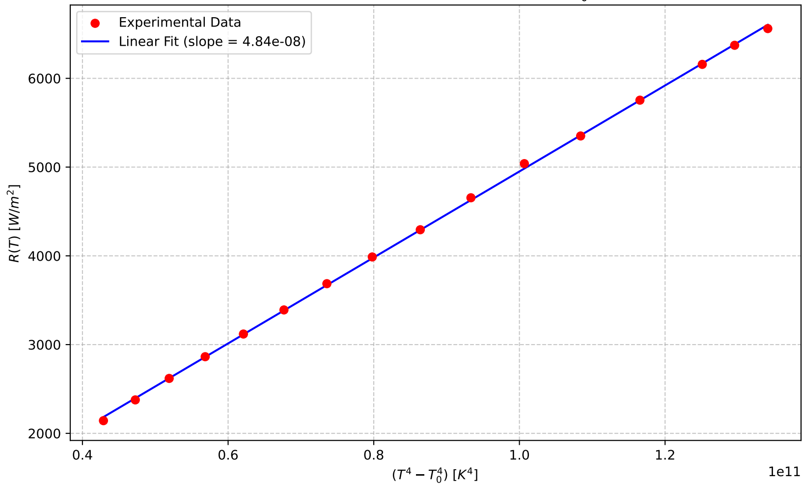
Stefan-Boltzmann Law: R(T) vs. (T^4 - T_0^4)
