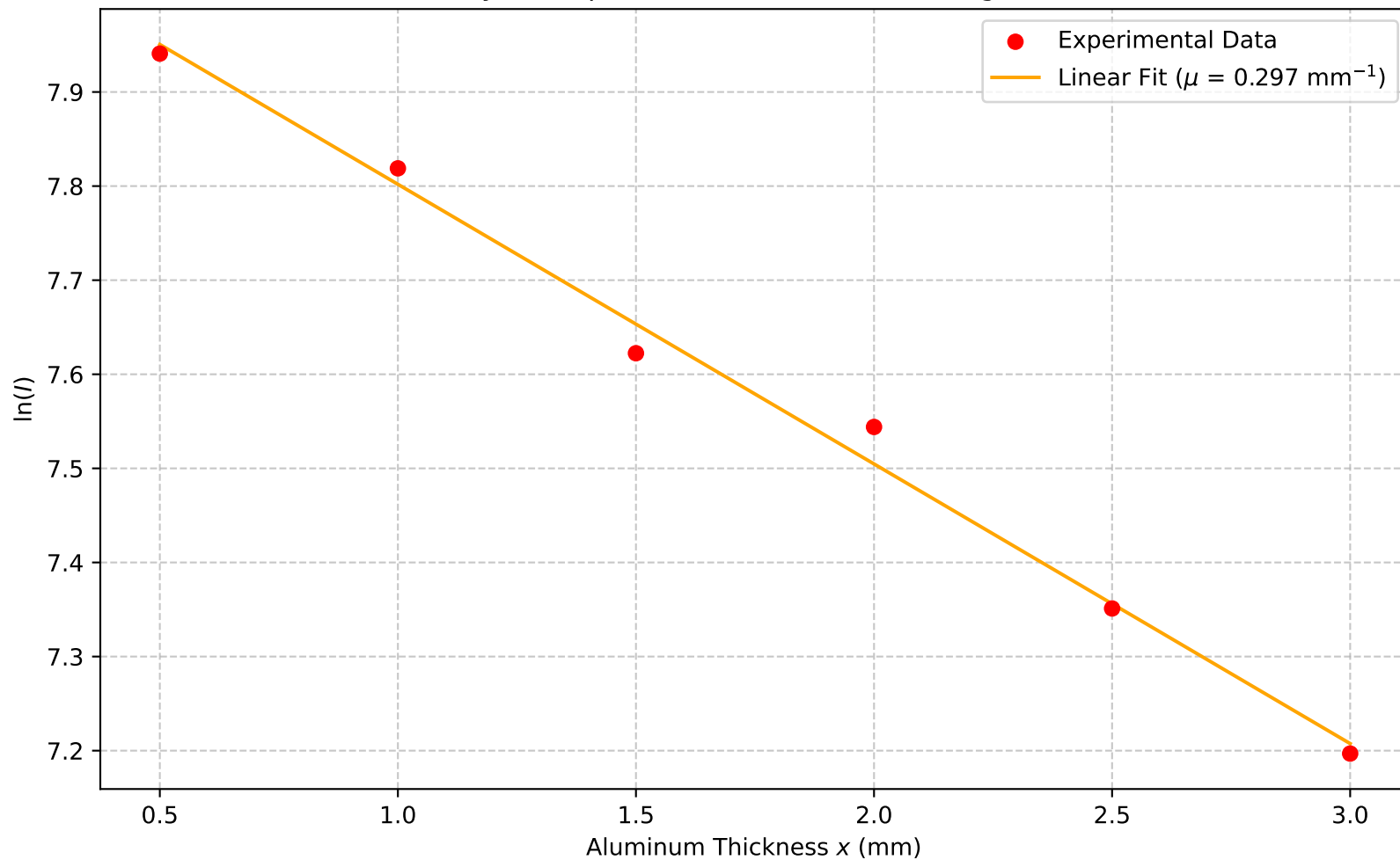
X-Ray Absorption in Aluminum (Semi-Log Scale)
