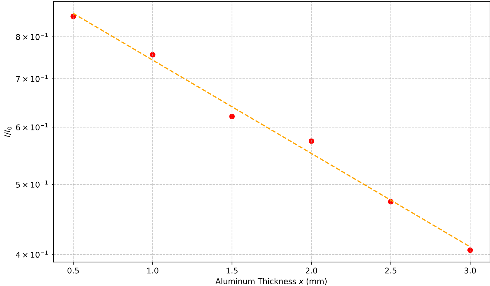
Normalized Transmission I/I_0 in Aluminum
